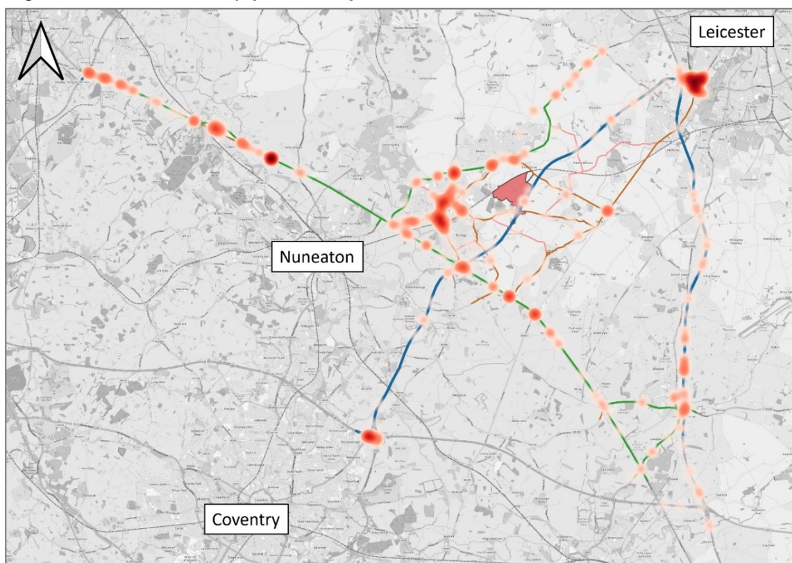
Figure 3.2: Collision Heatmap (2020 – 2023)
